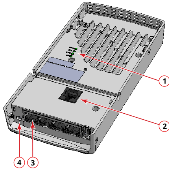
FIGURE 2 H550 Rear and bottom view
